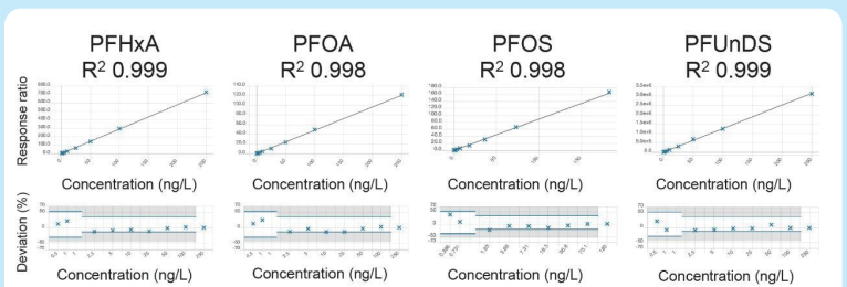
Figure 1. Calibration data of four PFAS compounds demonstrating calibration curve linearity and calibration deviation.
